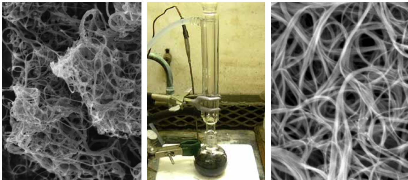
Single-walled Carbon Nanotube Purification: The image on the left shows raw SWCNTs, a naturally occurring allotrope of carbon. Through a purification process using acid reflux (shown center) and thermal oxidation, the NPRL is working to improve and verify the quality and consistency of the material. Research shows the purified material (right) provides greater efficiency in technologies like lithium ion batteries.
