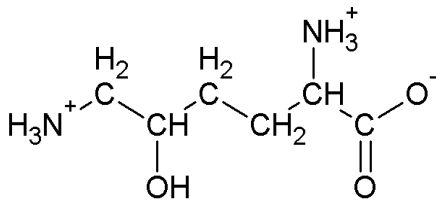
5-Hydroxylysine
