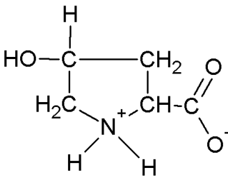
4-Hydroxyproline
