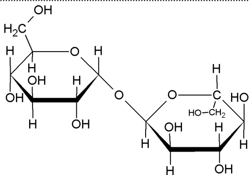
Lactose ( \beta form) \beta -D-galactopyranosyl-(1 \rightarrow 4)- \beta -D-glucopyranose Gal( \beta 1 \rightarrow 4)Glc
