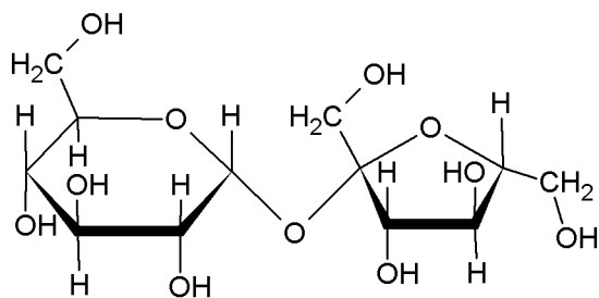
Sucrose \alpha -D-glucopyranosyl \beta -D-fructofuranoside Glc( \alpha 1 \leftrightarrow 2 \beta )Fru
