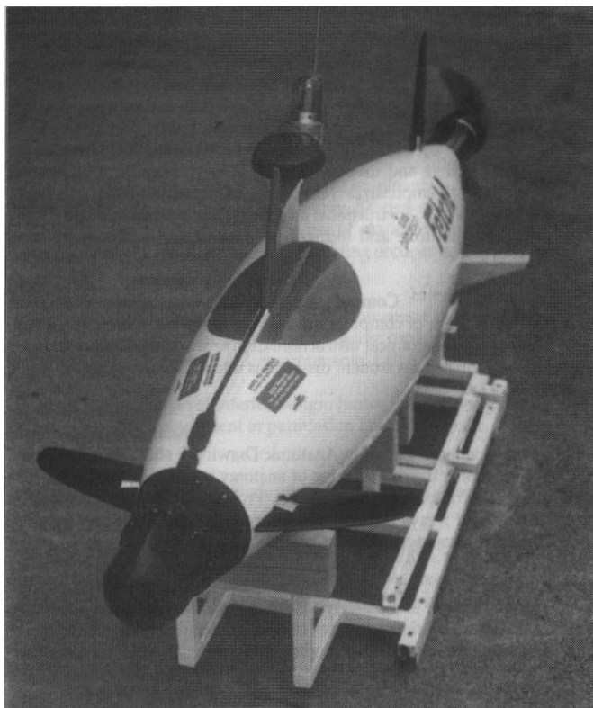
Fetch!, an autonomous underwater vehicle created by industrial design professor Jim Sias and collaborator Mark Patterson, could revolutionize underwater exploration. Replacing clunky ship-tethered devices, Fetch! is portable, weighs just 170 pounds and is computer controlled.
