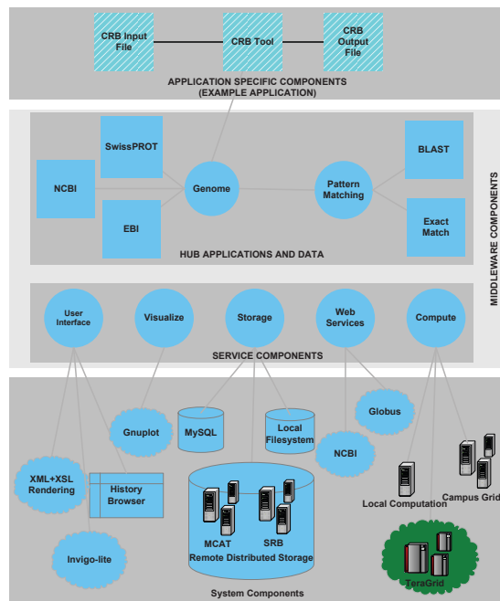
Fig. 3. The component hierarchy of SALSAs.
