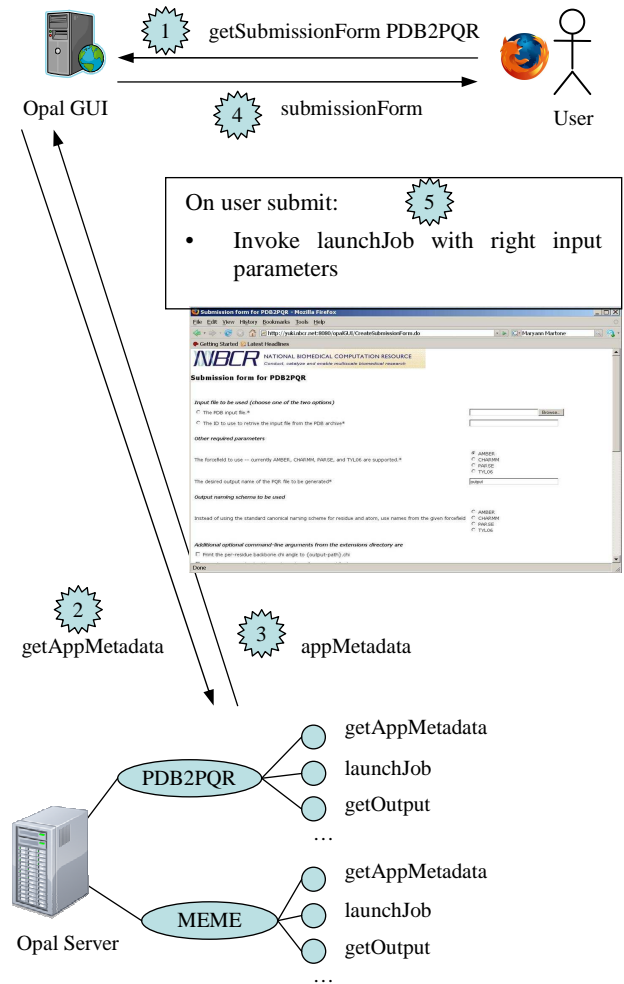
Figure 1 - Service invocation with Opal GUI
