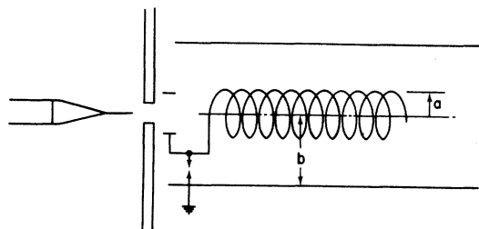
Fig. 5. Slow wave helix experiment.
