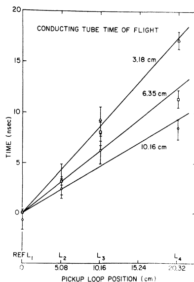
Fig. 3. Beam time of flight vs. pickup loop position.
