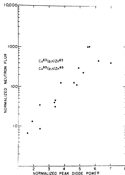
Fig. 2. Neutron flux vs. peak delivered power to the diode.
