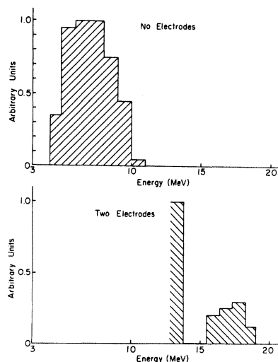
Fig. 4. Proton energy spectra with and without floating electrodes.
