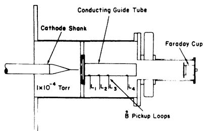
Fig. 1. General experimental configuration.
